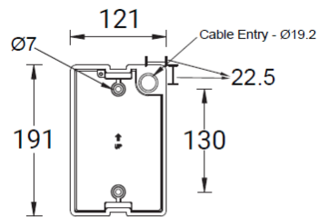
Mounting Plate
